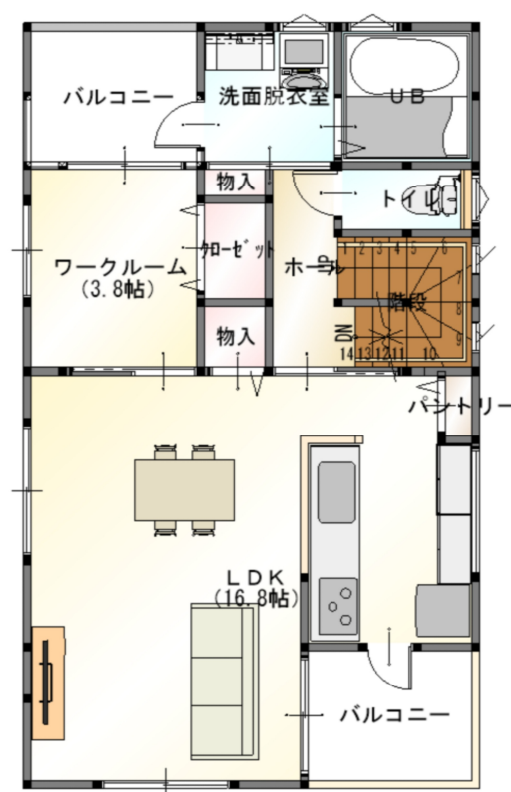
2F PLAN
