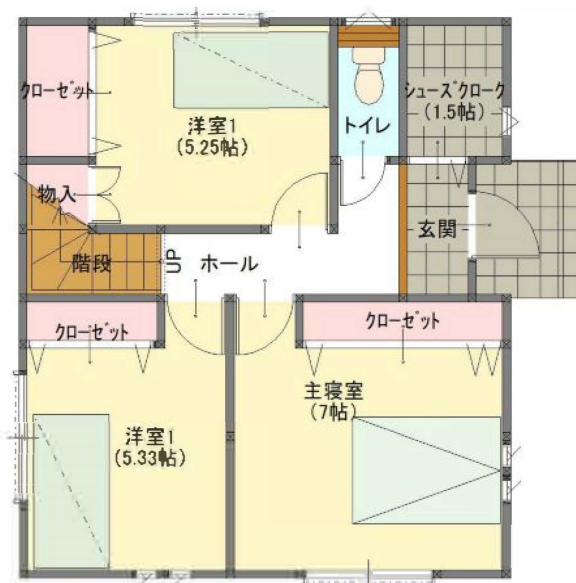
1F PLAN
