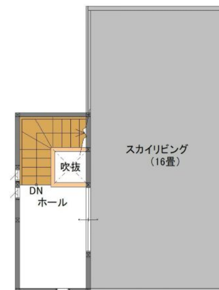
PHF PLAN
