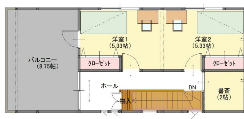
3F PLAN
