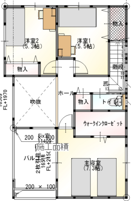
■ 2F PLAN
